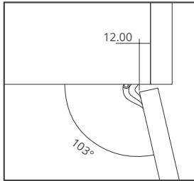
DOOR PROJECTION
