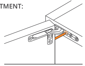
LATERAL ADJUSTMENT: +2mm / -2mm
