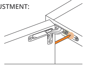
VERTICAL ADJUSTMENT: +1,5mm / -1,5mm
